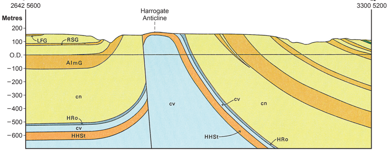
Geological section along the line P – Q
